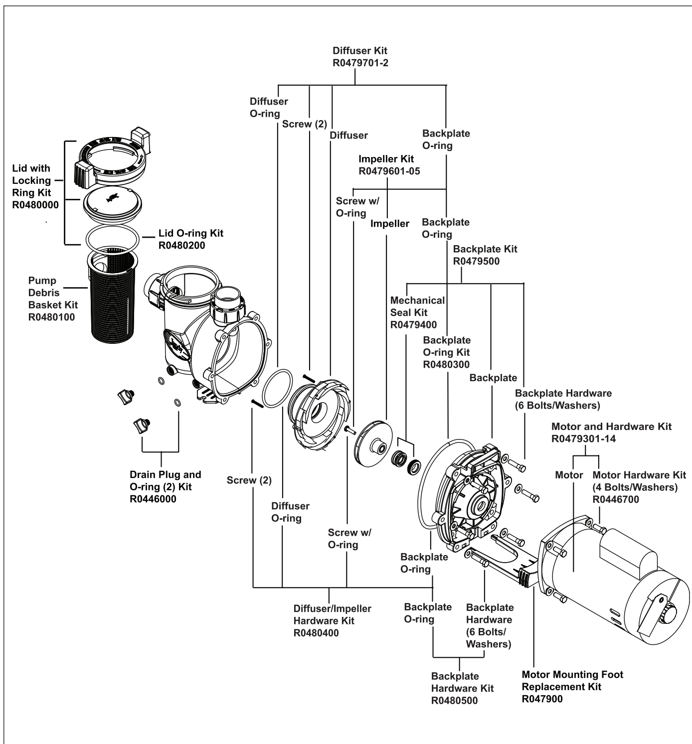
Figure 9. FHP Pump Parts Replacement Kits
