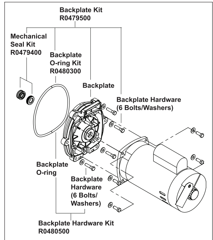
Figure 4. Backplate, Hardware, and Mechanical Seal Kits
