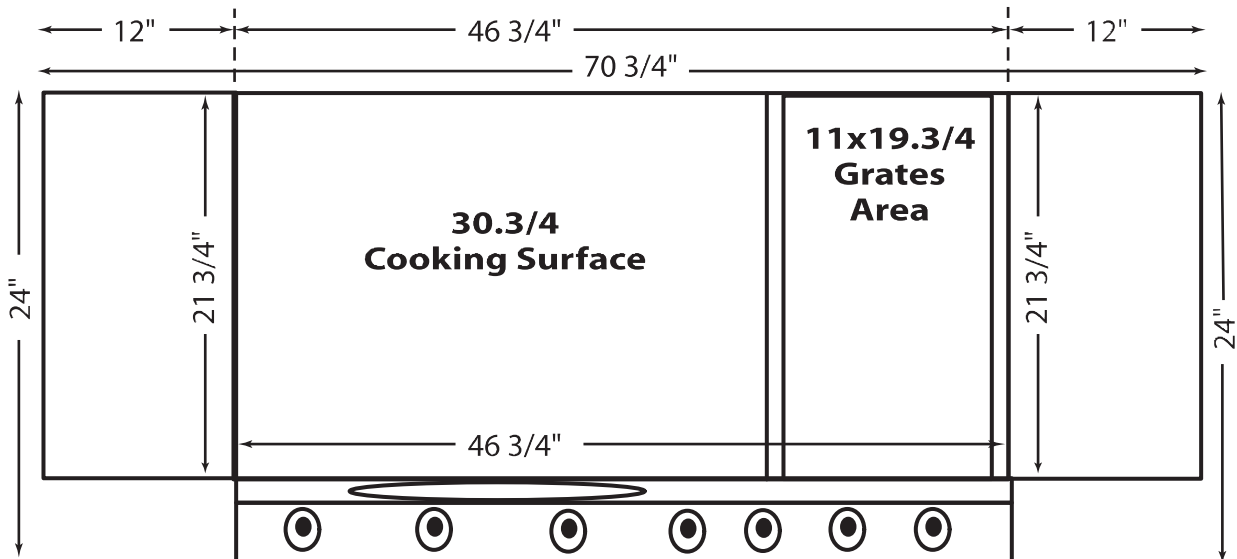
Top View
