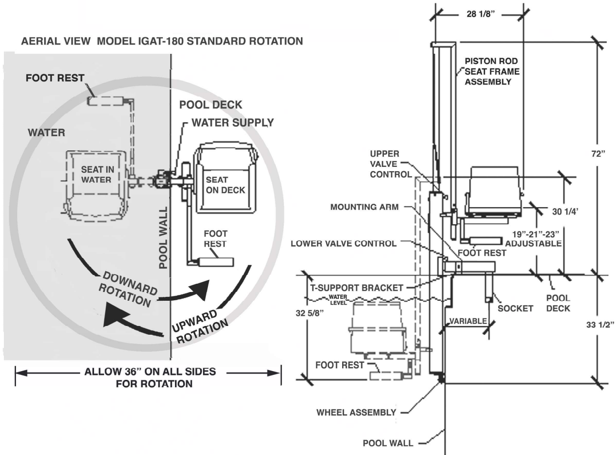
SIDE VIEW MODEL IGAT-180 STANDARD ROTATION
