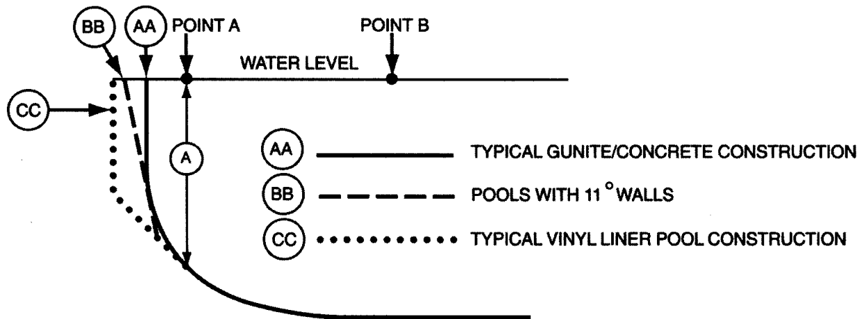
Figure 1- Maximum allowable wall slope
