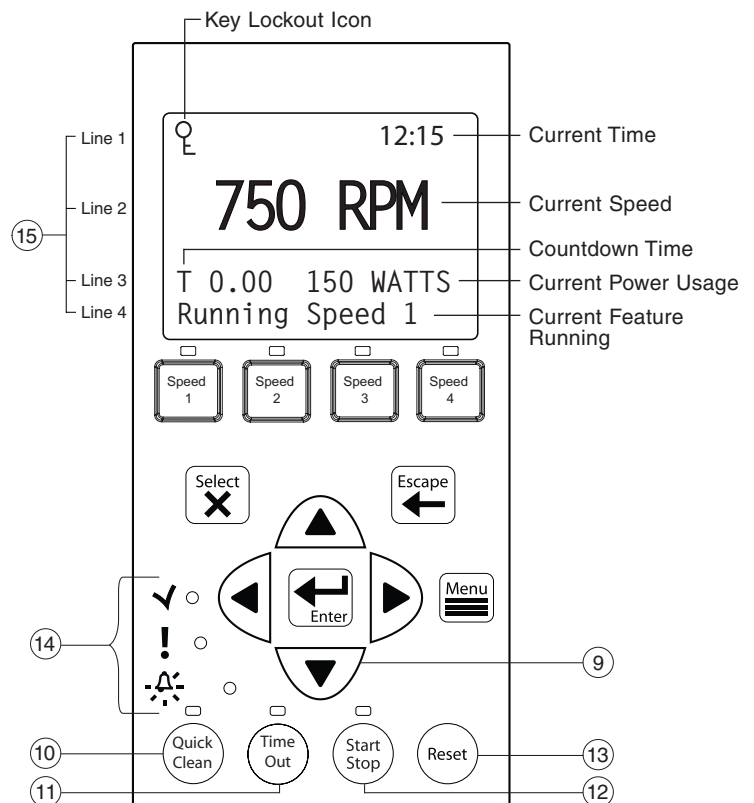
Control Panel #9-15
