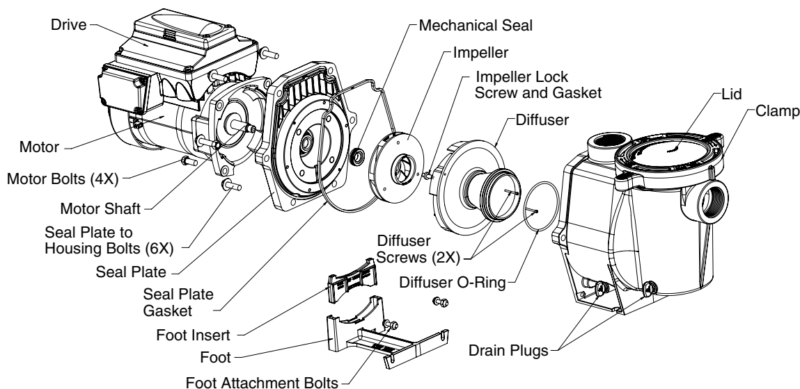
Pump Exploded View
