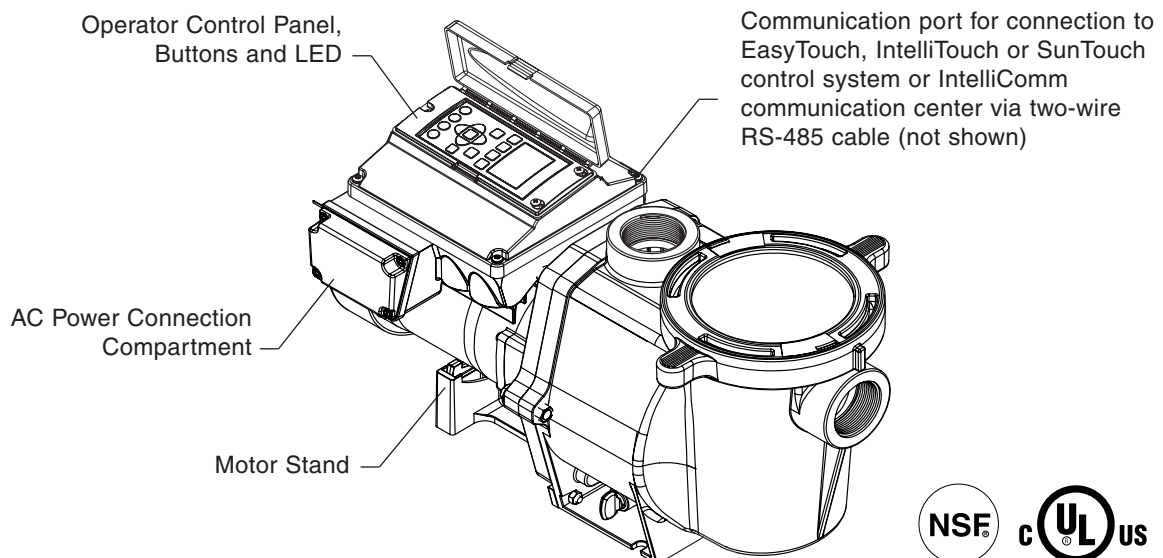
IntelliFlo i1 Variable Speed Drive Assembly
