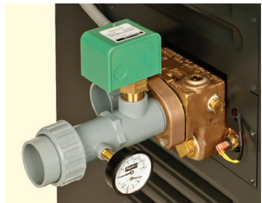
Flow switch and T&P gauge-standard
