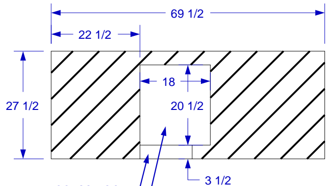
ACCESS DOOR UTL STUB-UP AREA
