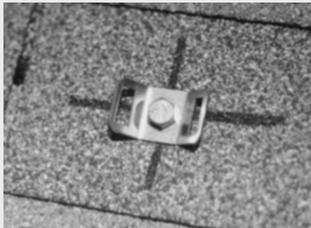
FIGURE 6 Strap Bracket
