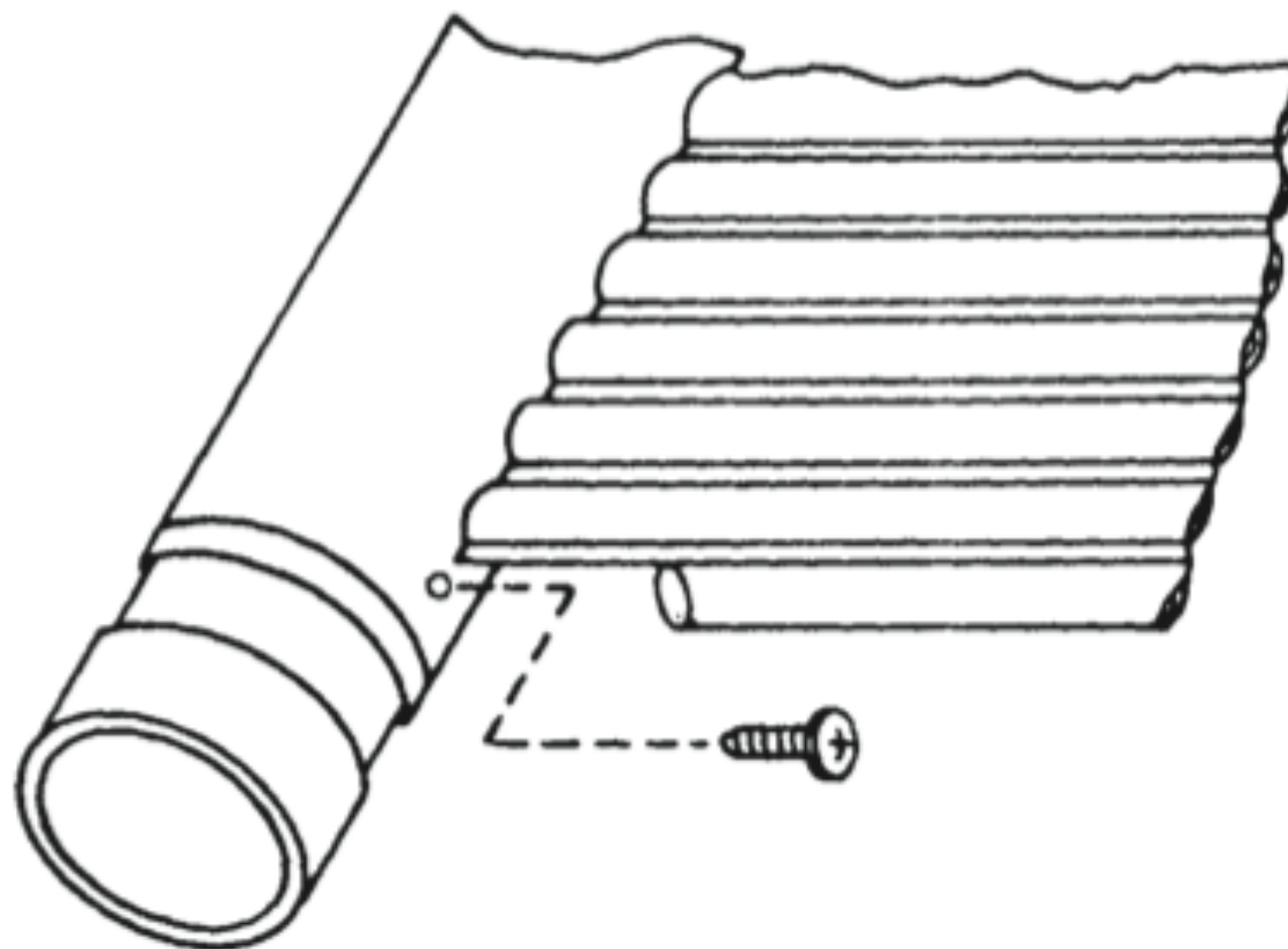
FIGURE 16 Collector Repair
