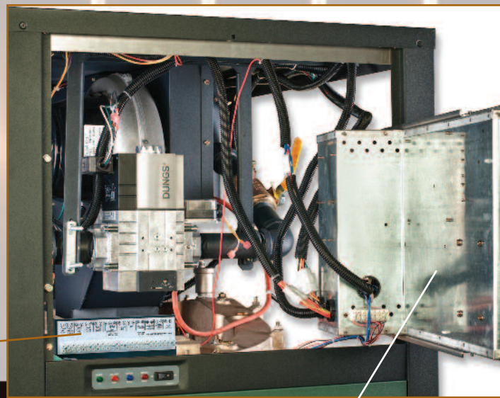
Control panel swings open for easy control access.
