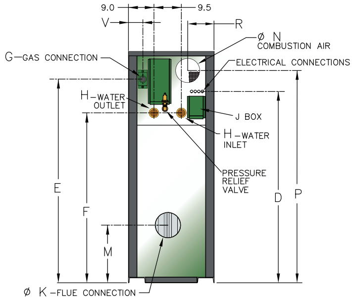
REAR VIEW
