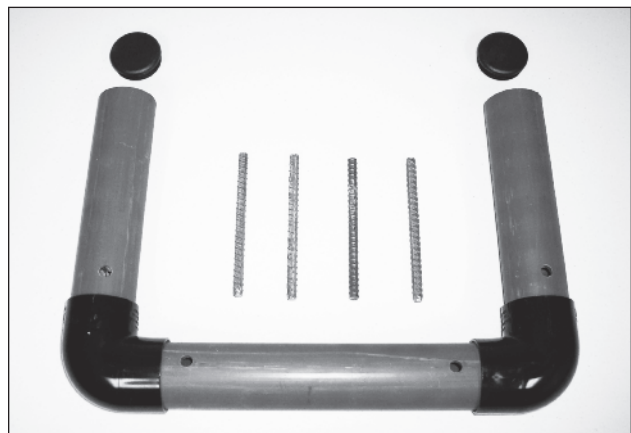
Fig. 2 Plastic Anchor Jig for In Deck Installation
