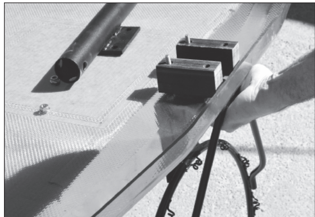
Fig. 23 Rim Assembly
