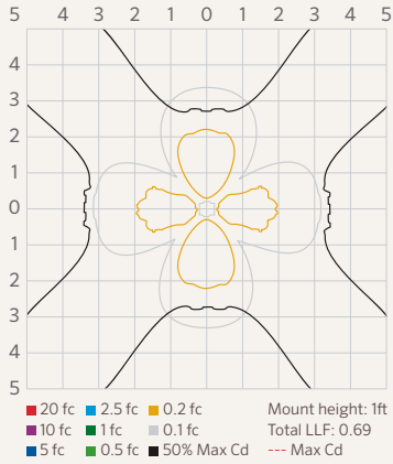
FC 1LED ISOFOOTCANDLE PLOT
