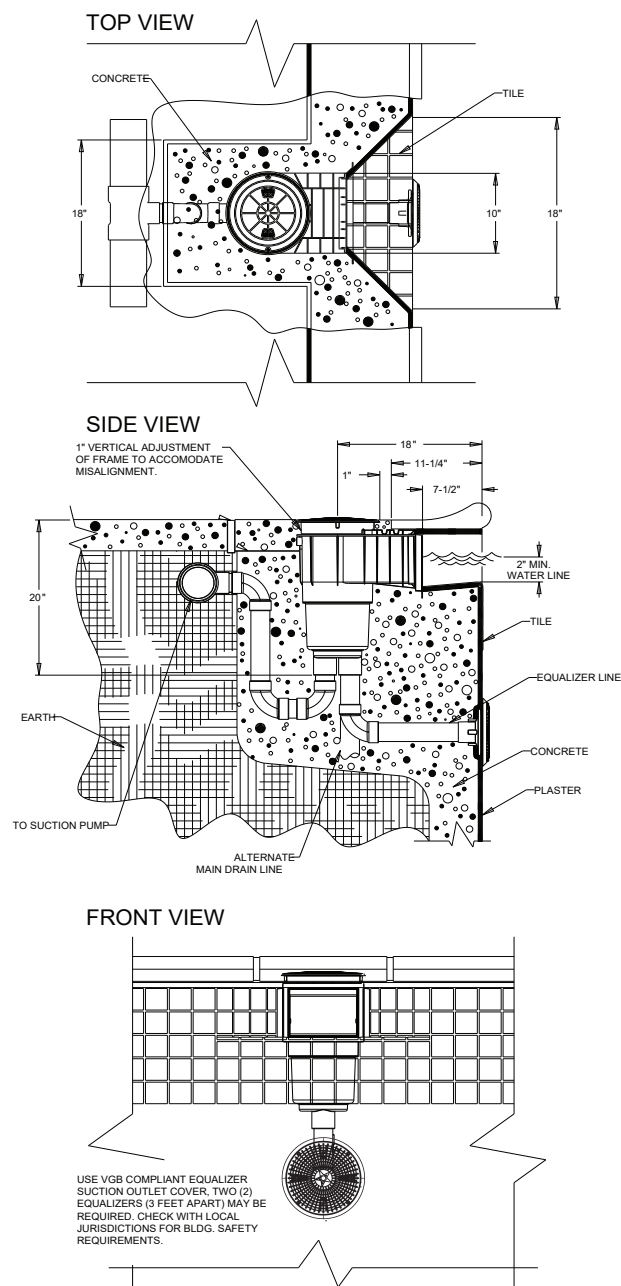
Figure 7: SKR1xxx skimmer installation drawings and specifications.
