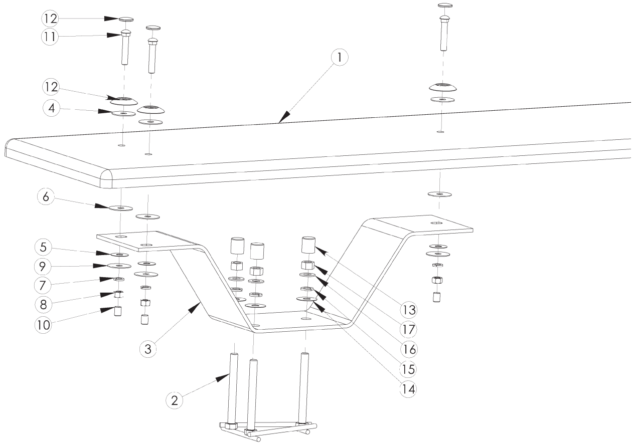
DRAWING REPRESENTS THE FOLLOWING PART NUMBERS: DSS6 (shown) DSS8
