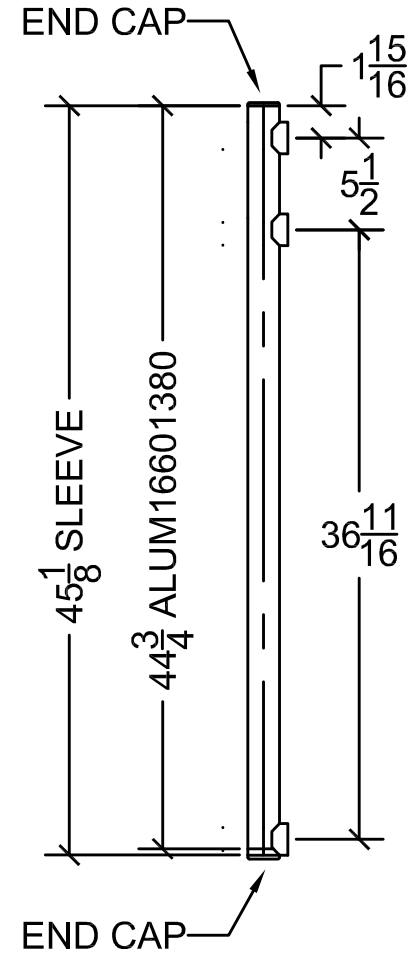
QTY: 2 GATE POST
