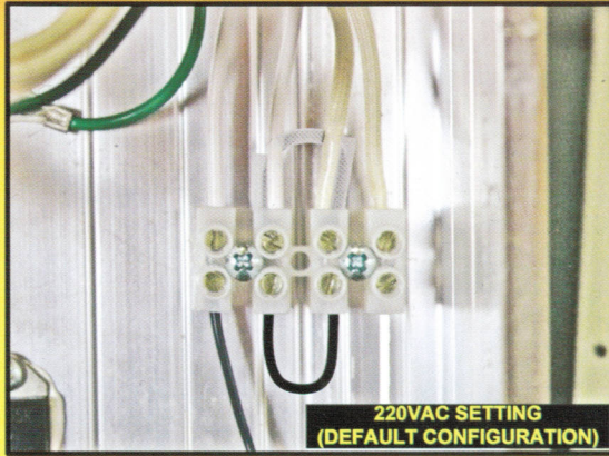
Figure 3 – 220 VAC Configuration
