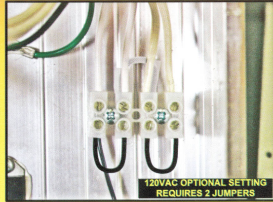
Figure 4 – 120 VAC Configuration
