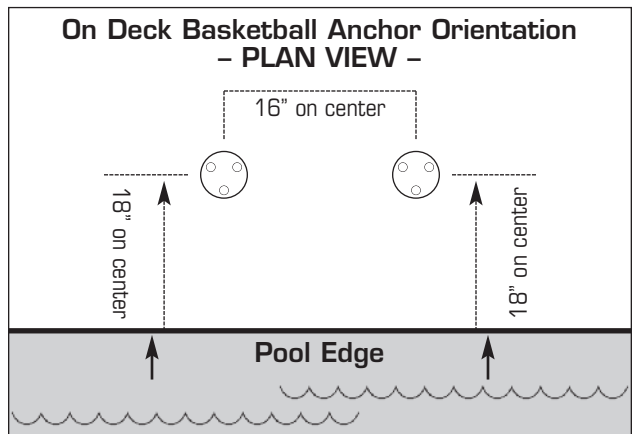
Fig. 29 On Deck Anchor Orientation
