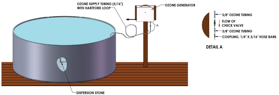
Figure 2. Standard Installation Diagram
