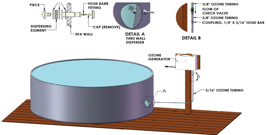
Figure 3. Thru-Wall Dispenser Installation Diagram
