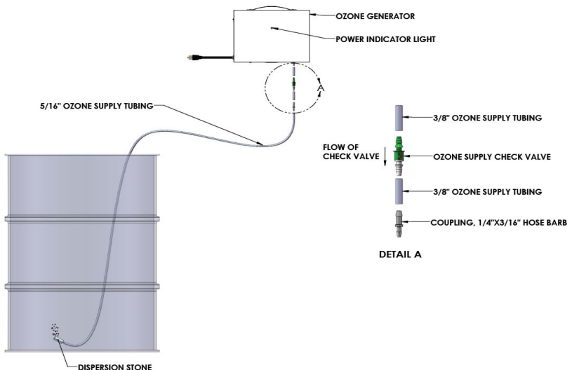
Figure 1. Example Installation Diagram
