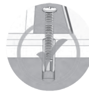
FIGURE 4 ENSURE AT LEAST THREE THREADS OF ENGAGEMENT AND HAND CHECK TO ENSURE SCREW IS SECURE
