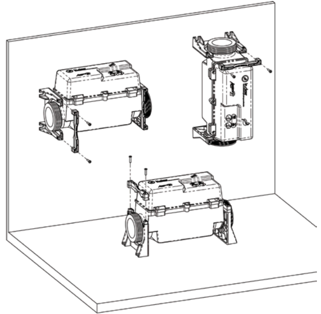
Floor and side mounting
