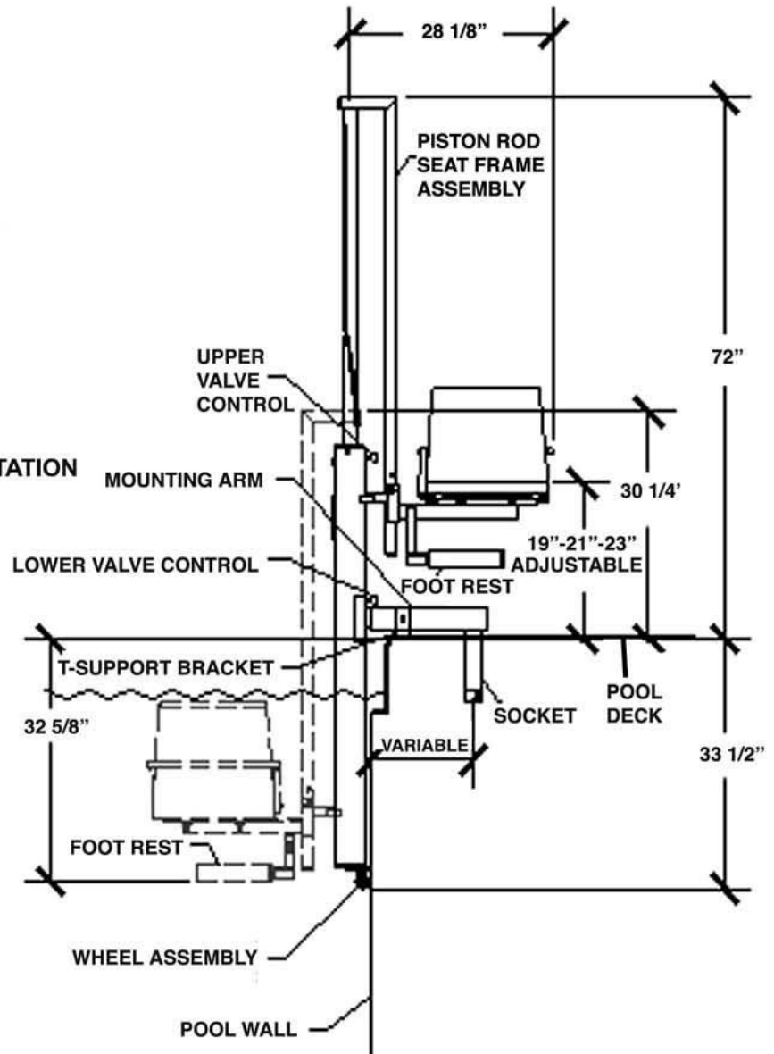
SIDE VIEW MODEL IGAT-180/135 STANDARD ROTATION
