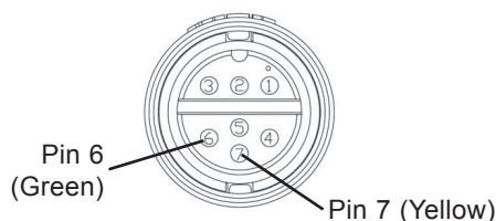
Pump cable pin configuration
