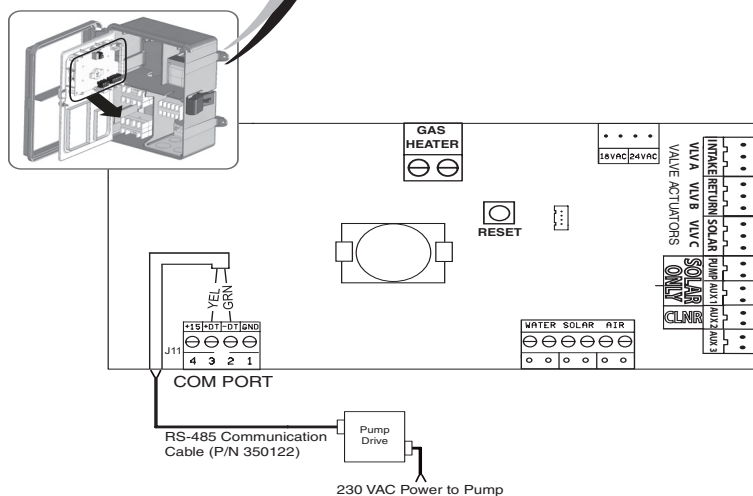
SunTouch System Motherboard
