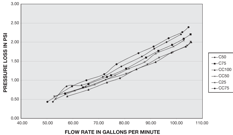
HEAD LOSS CURVE : TRIMLINE CARTRIDGE FILTER
