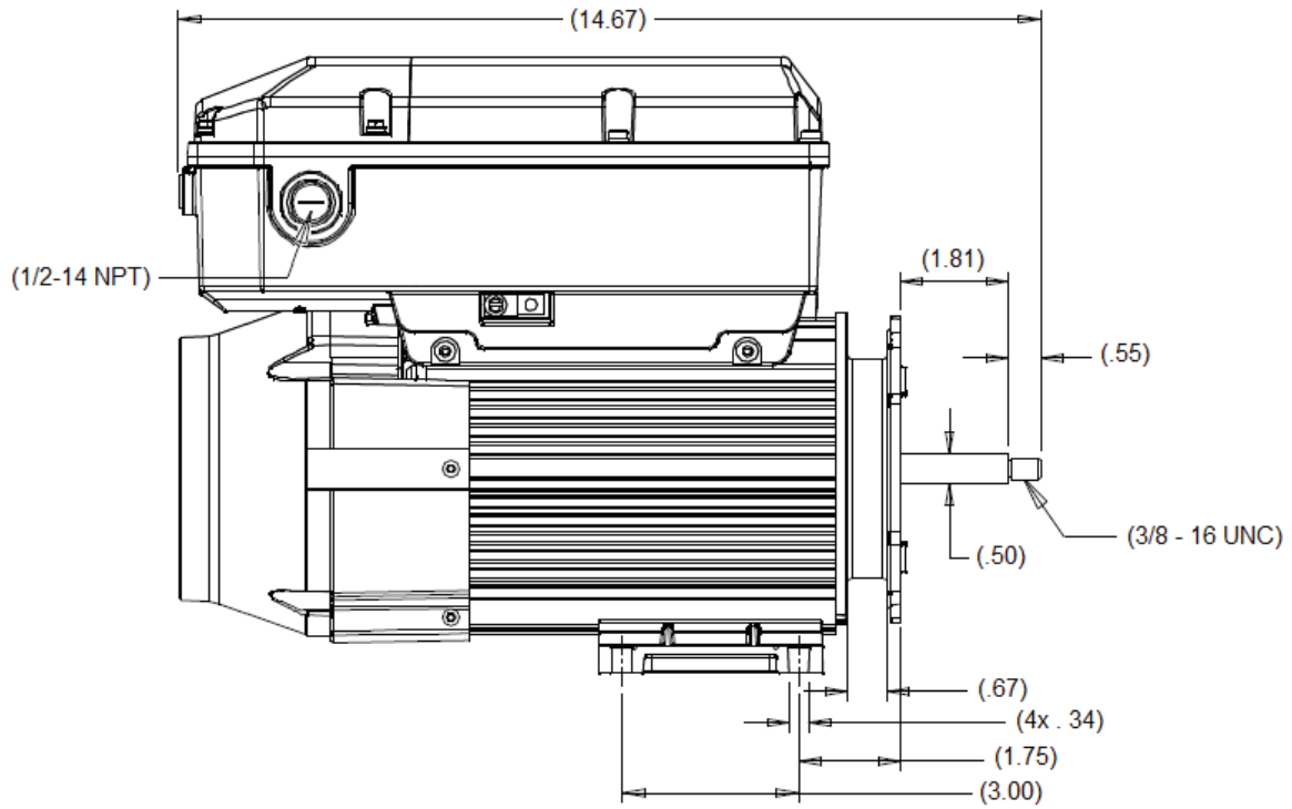
Side View
