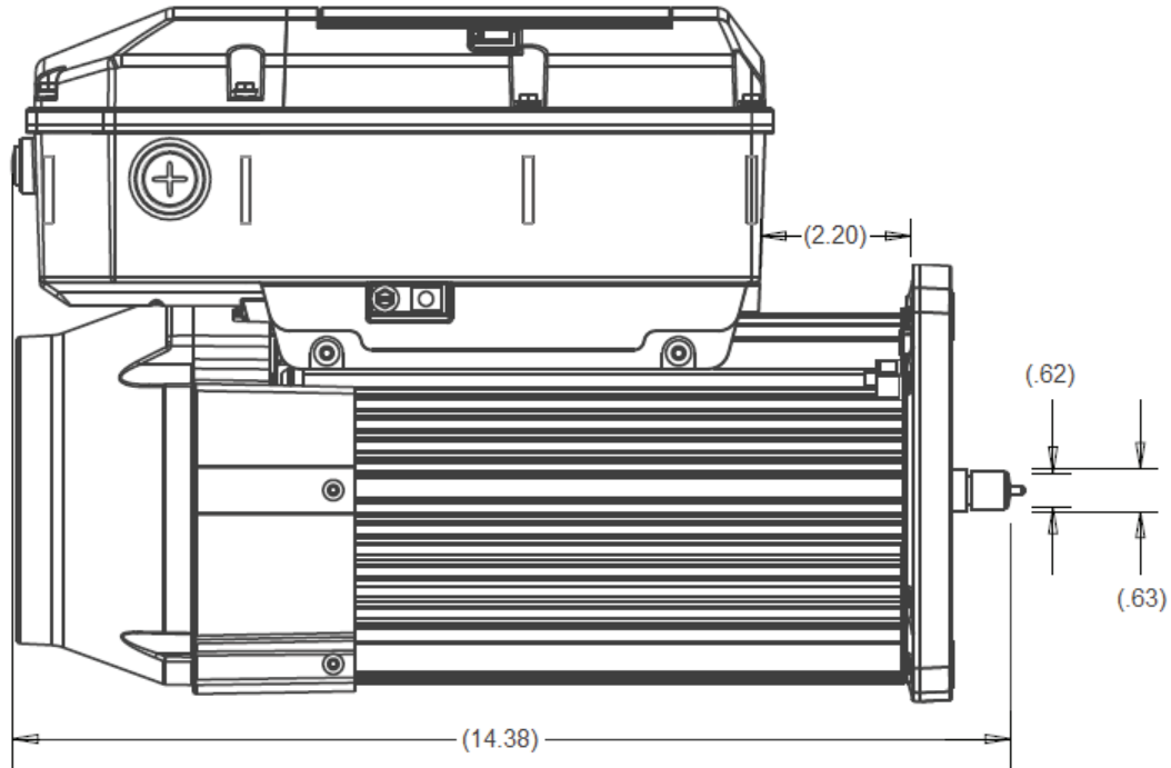
Side View
