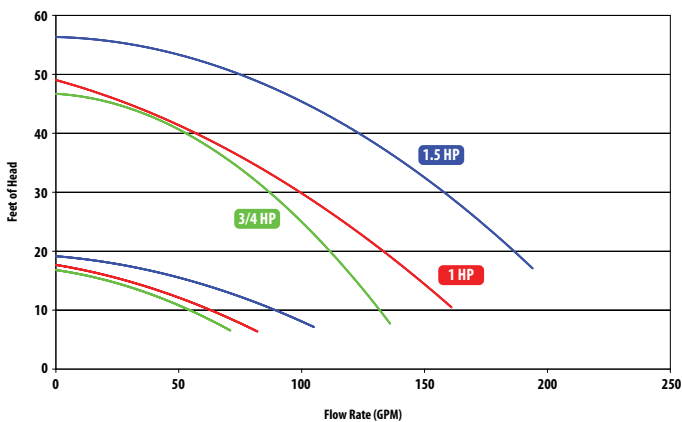
Hi-Flo Pumps - Performance Curves
