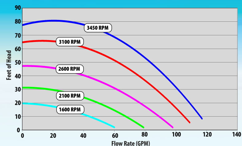
Power Defender – 1.65 HP – Performance Curves
