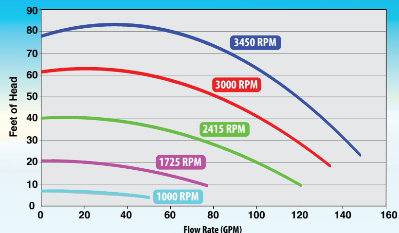
Power Defender 270 – 2.7 HP – Performance Curves
