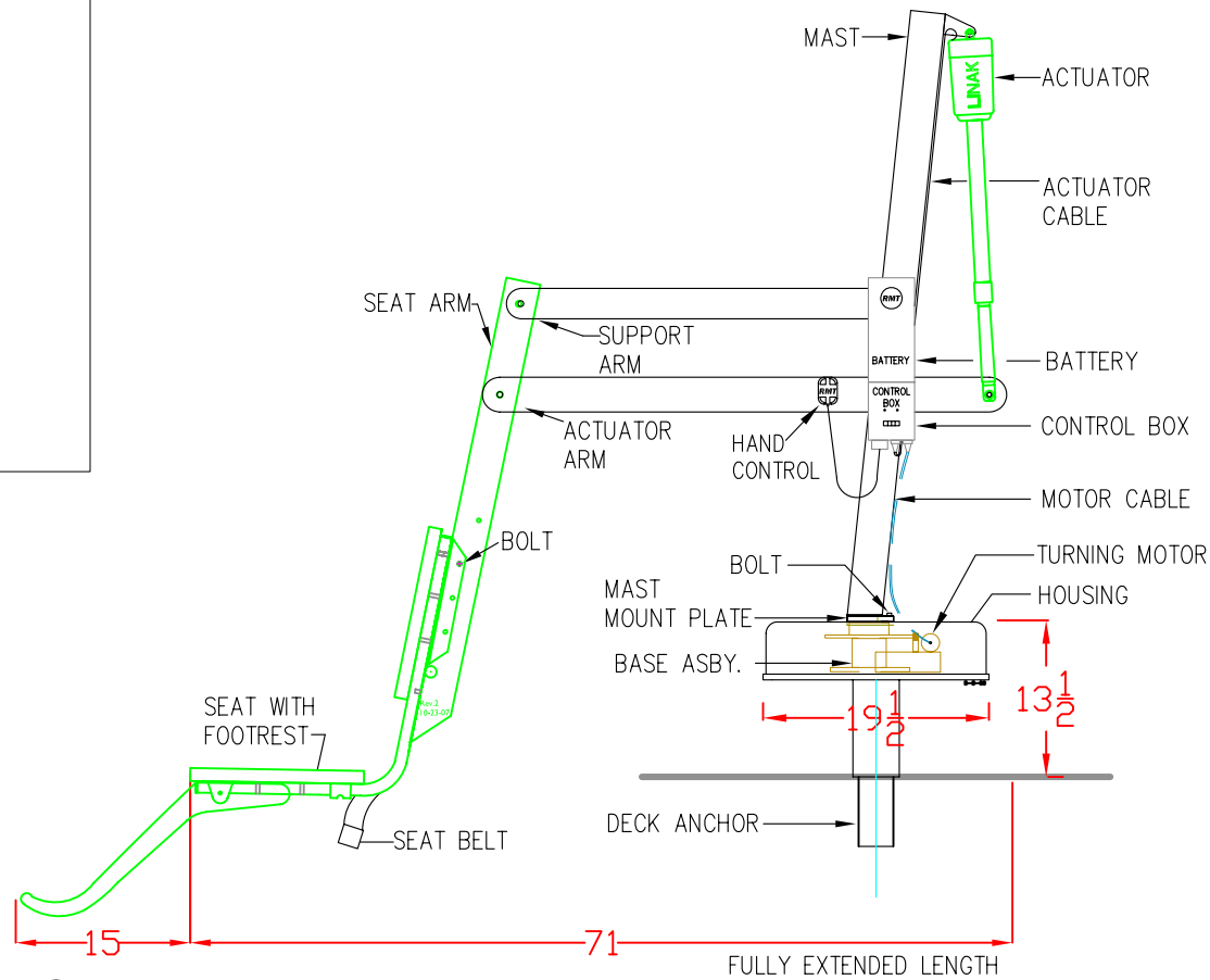
SPLASH!-SIDE VIEW COMPONENT IDENTIFICATION 5-5-09 FINAL
