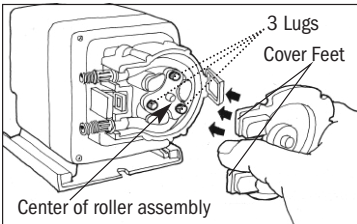
D Align cover feet near tube fitting
