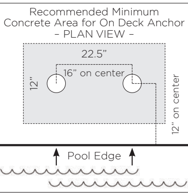
Anchor Placement - Plan View
