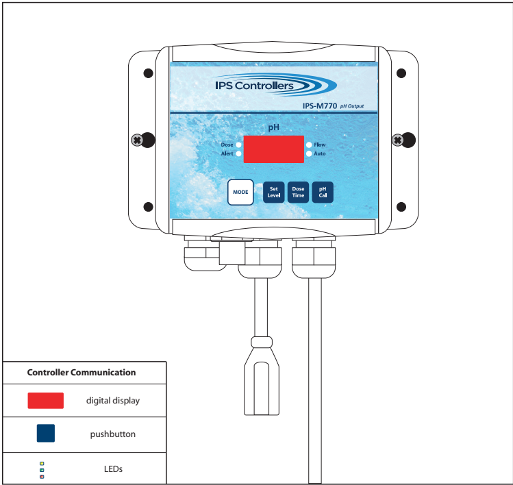
Figure 2: M770 Controller Components Connections
