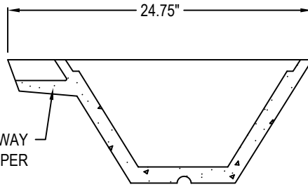
SIDE SECTION
