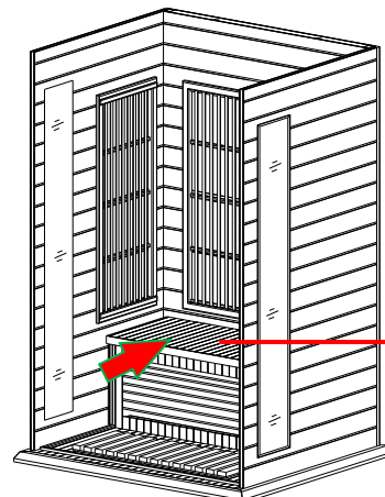
FIG 10 Installing Bench
