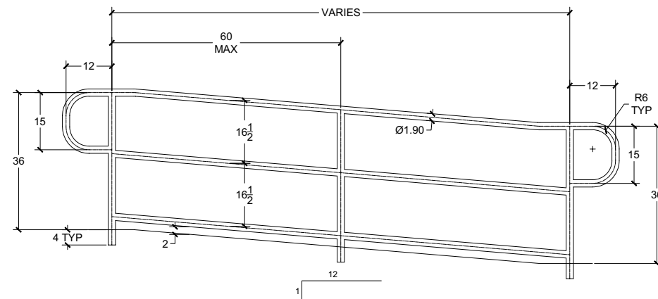
3 RAIL ADA RAMP RAIL CAN ALSO LEVEL OUT TO POST WITH NO P-LOOP
