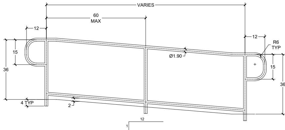
2 RAIL ADA RAMP RAIL CAN ALSO LEVEL OUT TO POST WITH NO P-LOOP
