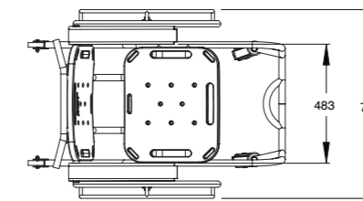
Seat is 381mm deep and 457mm wide
