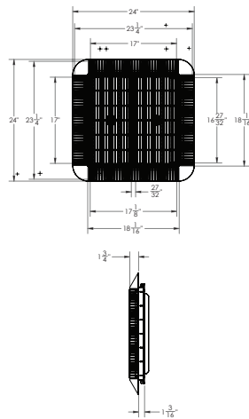
Standard Adapter Frame for 1" deep Standard 12" square mud frames
