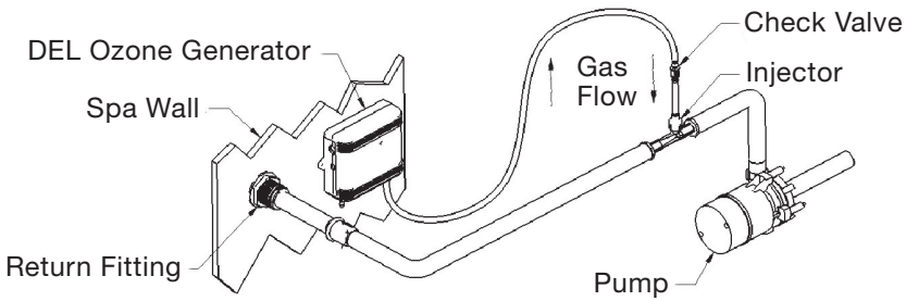
Figure 4 Typical Injection System
