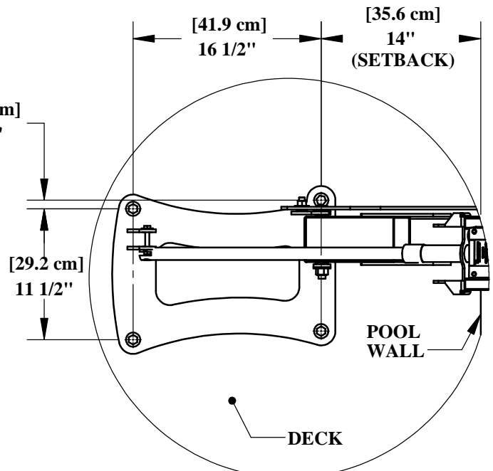
ANCHOR BOLT PATTERN
