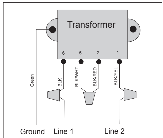
Figure 3. Factory Wiring for 220 Volt Operation
