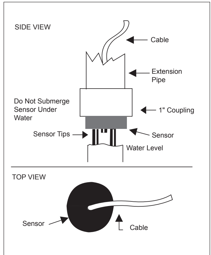
Figure 8. Slip Sensor on Static Pipe
