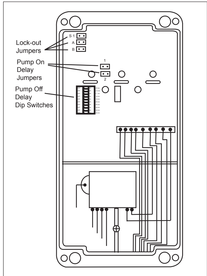
Figure 13. Jumpers and Dip Switches
