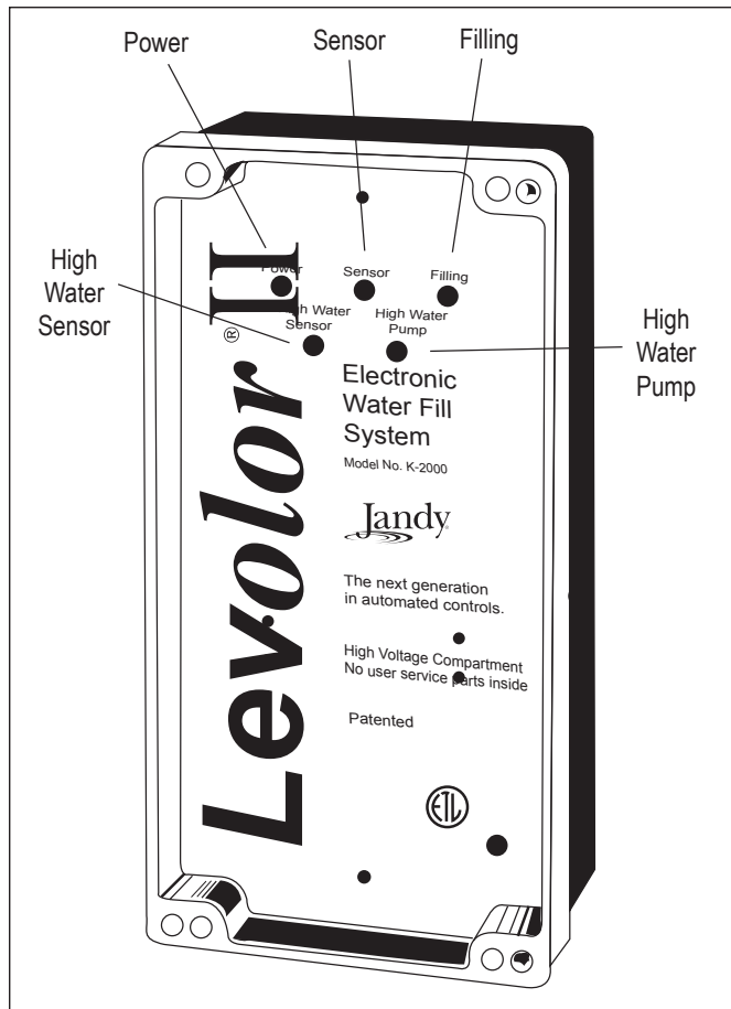
Figure 12. Controller Lights
