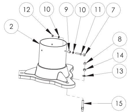
DETAIL D
