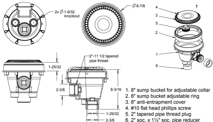
Part # 8SBACxxx
