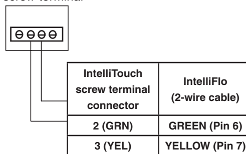
Pin configuration
