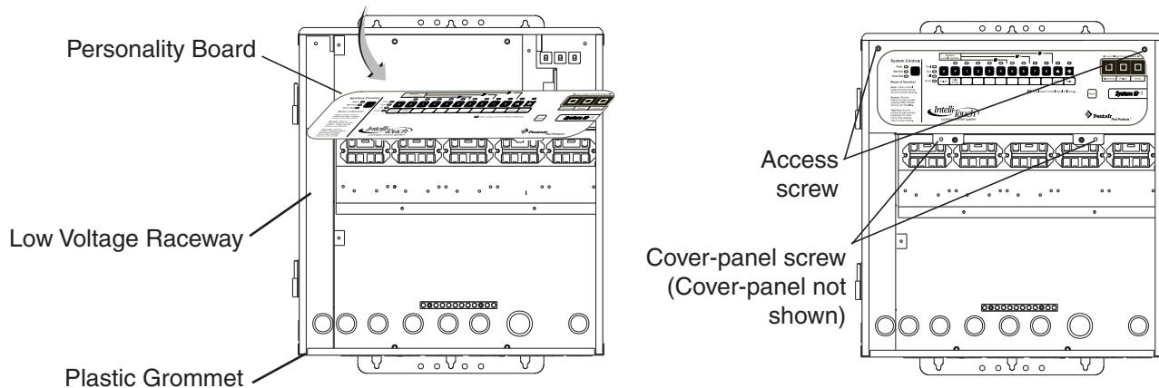
IntelliTouch Control System Load Center
