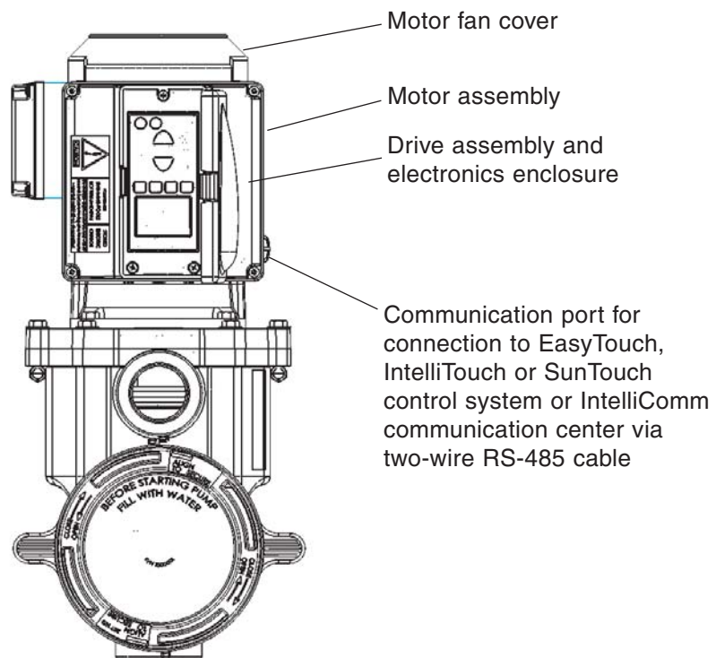
IntelliFlo VF (variable flow pump)
