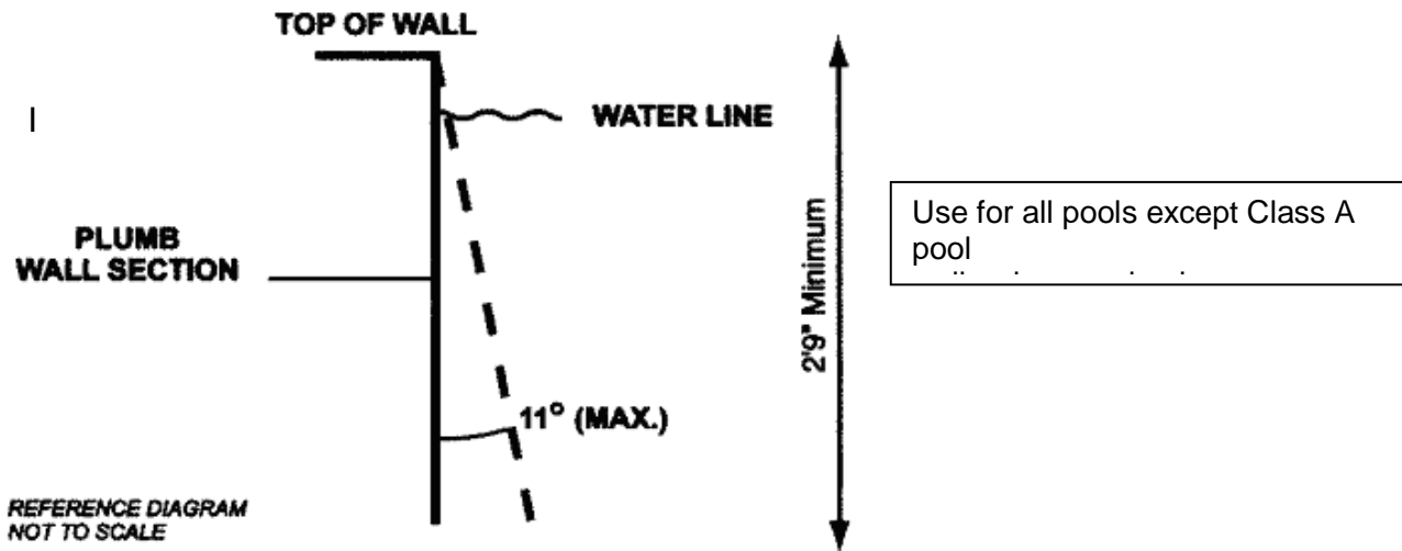
Figure 2 – Maximum allowable wall slope
