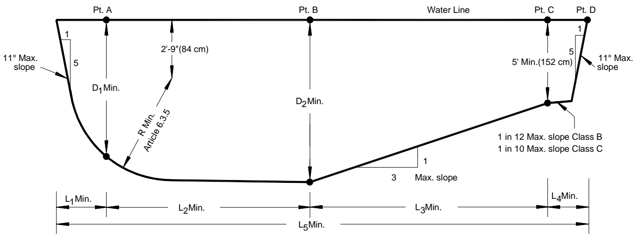
Figure 1 – Construction dimensions for water envelopes for Class B and Class C pools
